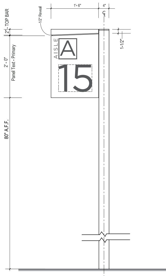
5 FRONT VIEW - SIDE A SCALE: 1" = 1'-0"
