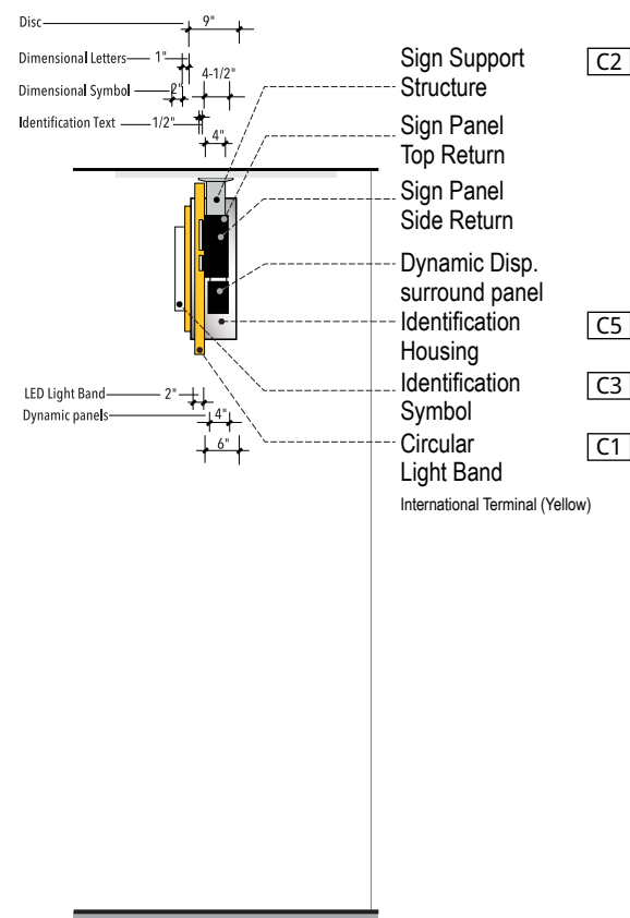
4 SIGN FINISHES - SIDE VIEW SCALE: NTS
