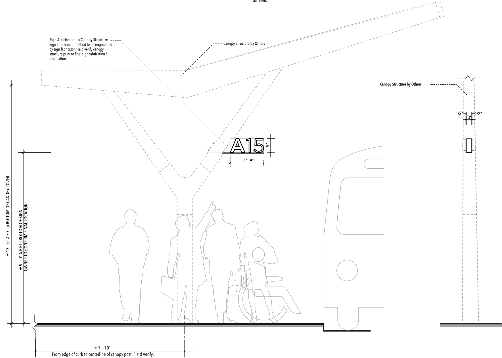
4 FRONT VIEW SCALE: 1/2" = 1' - 0"
