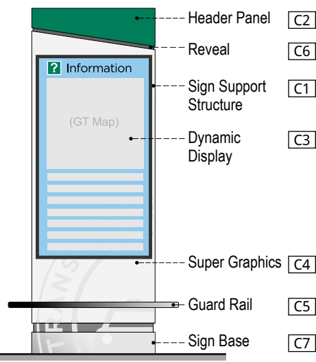
3 FINISH - FRONT VIEW SCALE: NTS
