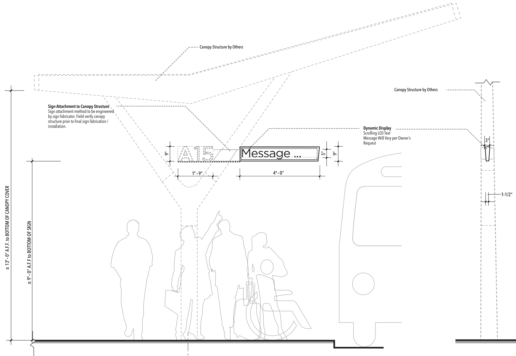
3 FRONT VIEW SCALE: 1/2" = 1'- 0"
