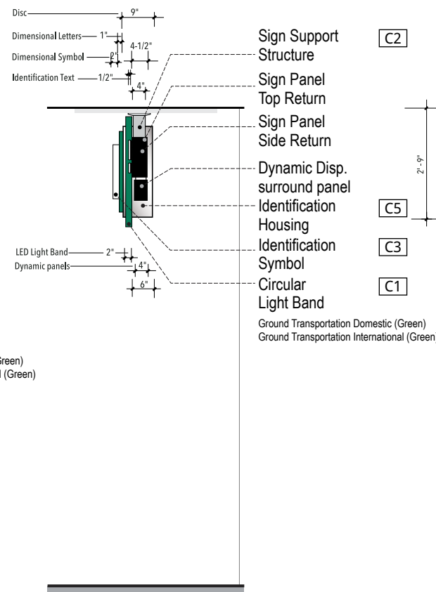
4 SIGN FINISHES - SIDE VIEW SCALE: NTS
