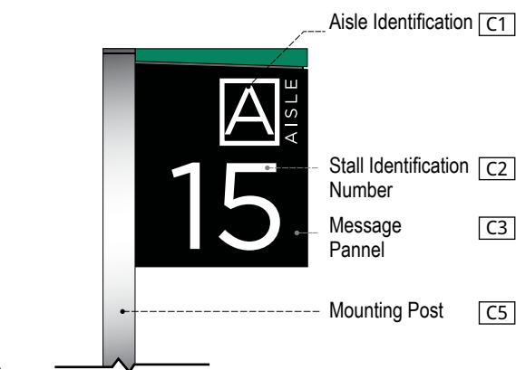
3 FINISH - FRONT VIEW SCALE: NTS
