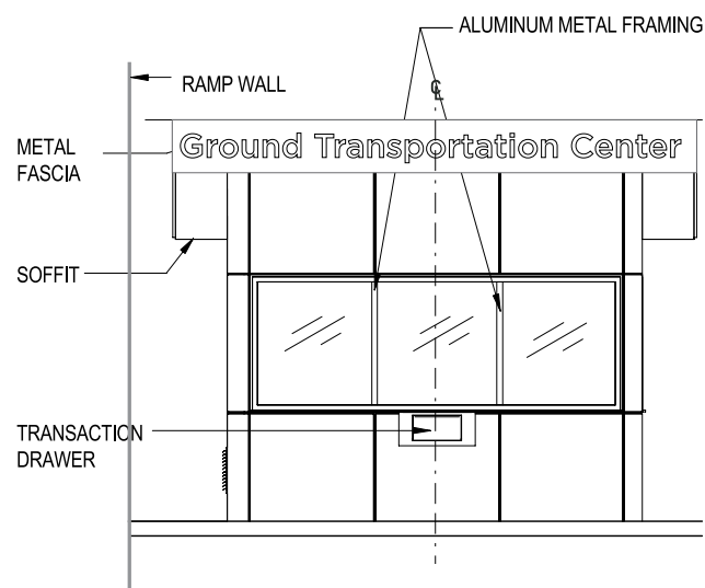
4 ELEVATION - BUILDING FRONT SCALE: NTS
