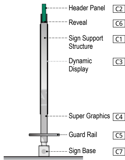
4 FINISH - SIDE VIEW SCALE: NTS
